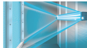
CX30 installed on a vertical coil
