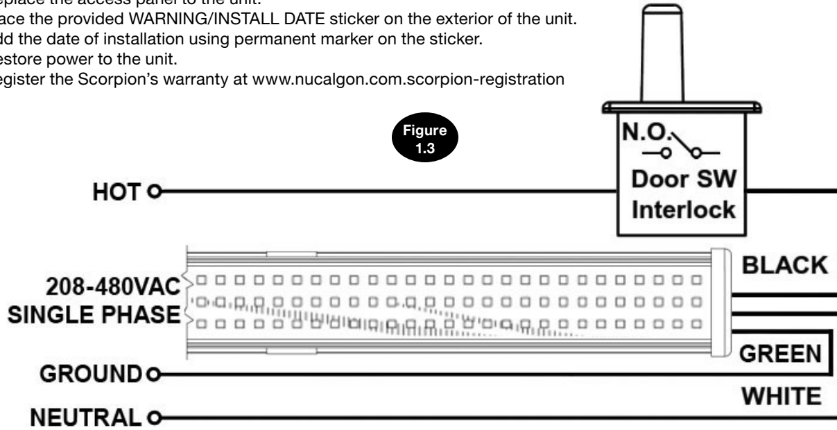
CX30 UVC-LED Wiring Diagram
